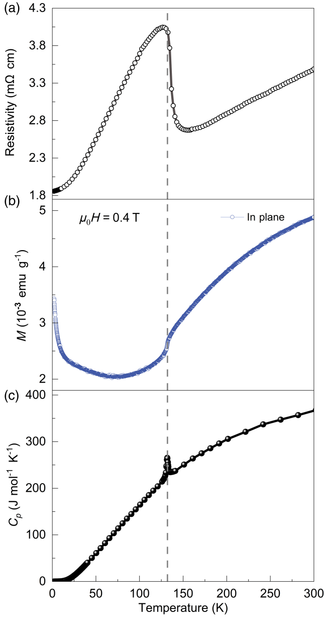
FIG. 2. Physical properties of La_4Ni_3O_{10} single crystals. (a) Temperature-dependent resistivity. (b) Temperature-dependent magnetization. (c) Temperature-dependent heat capacity.
