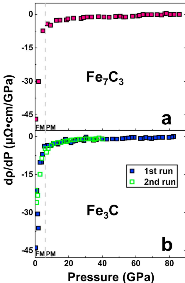
Figure 4. First-order pressure derivative of the electrical resistivity of (a) \text{Fe}_7\text{C}_3 and (b) \text{Fe}_3\text{C} ( dp/dP ) at high pressures. The drastic change in the derivative for \text{Fe}_7\text{C}_3 and \text{Fe}_3\text{C} at approximately 6 GPa is attributed to the ferromagnetic to paramagnetic (PM) transition reported previously (Chen et al., 2012, 2014; Duman et al., 2005; Gao et al., 2008; Litasov et al., 2013; Prescher et al., 2012). The flattening of the pressure derivative in the PM state indicates that the high-pressure effect on the electrical resistivity significantly decreases with increasing pressure.
