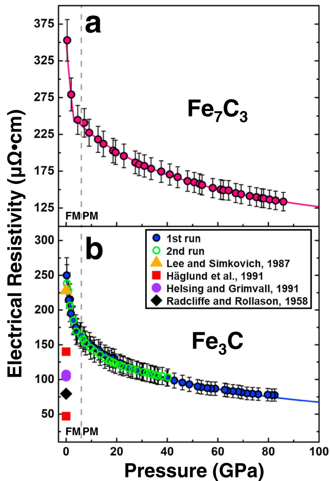
Figure 3. Electrical resistivity of (a) \text{Fe}_7\text{C}_3 and (b) \text{Fe}_3\text{C} at high pressures and room temperature. As shown by the vertical gray dashed lines, \text{Fe}_7\text{C}_3 and \text{Fe}_3\text{C} undergo the ferromagnetic to paramagnetic (PM) transition at \sim 6 GPa, respectively, such that the resistivity of each state has been modeled independently (shown as solid magenta and blue lines). The modeled results of the PM state are used for further high-pressure modeling of Earth's core P-T conditions. Circles: \text{Fe}_7\text{C}_3 (solid magenta circles), first run (solid blue circles), and second run (green open circles) for \text{Fe}_3\text{C} in this study; orange triangle: \text{Fe}_3\text{C} at ambient conditions (Lee & Simkovich, 1987); red squares, purple circles, and black diamond: previous calculated electrical resistivity of \text{Fe}_3\text{C} at ambient conditions (Häglund et al., 1991; Helsing & Grimvall, 1991; Radcliffe & Rollason, 1958).
